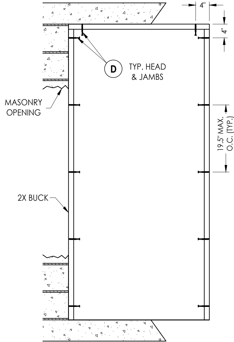
BUCK ANCHORING
