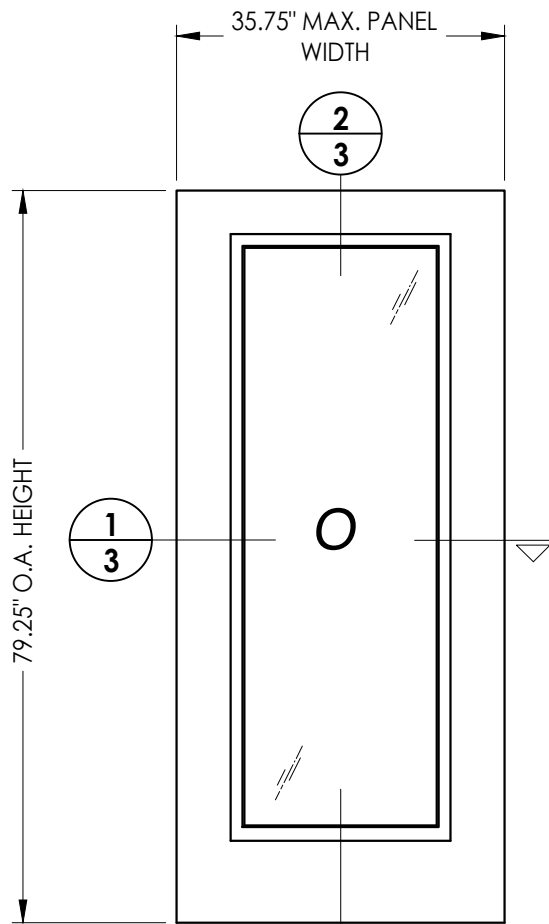
50 SIDELITE PANEL
