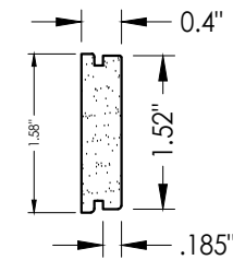
43 LATCH & HINGE STILE Cellular PVC
