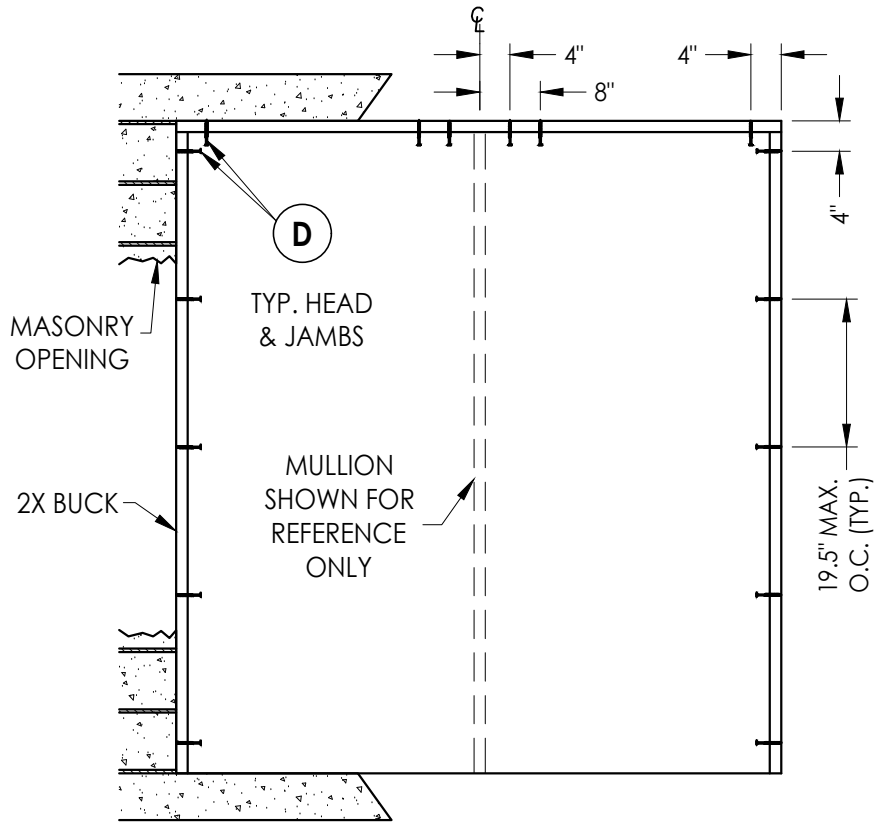
BUCK ANCHORING
