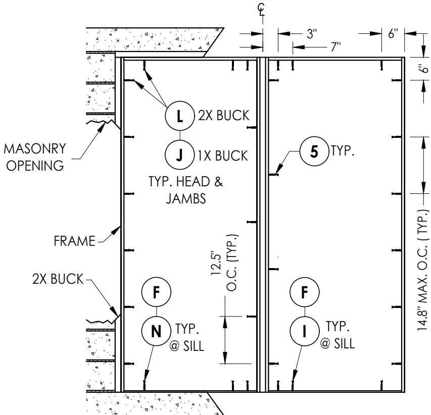
FRAME ANCHORING Masonry construction
