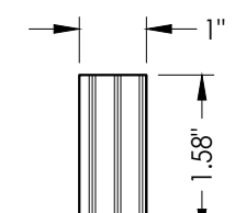
43 LATCH & HINGE STILE Cellular PVC
